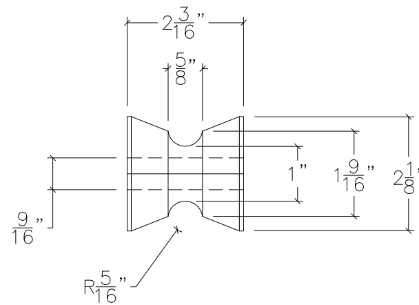
ROLLER #2
