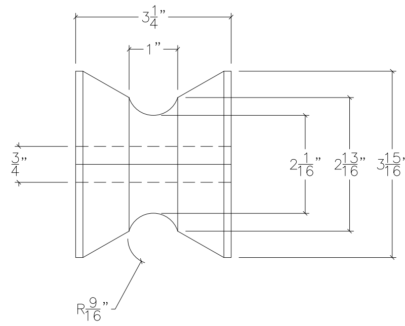
ROLLER #2
