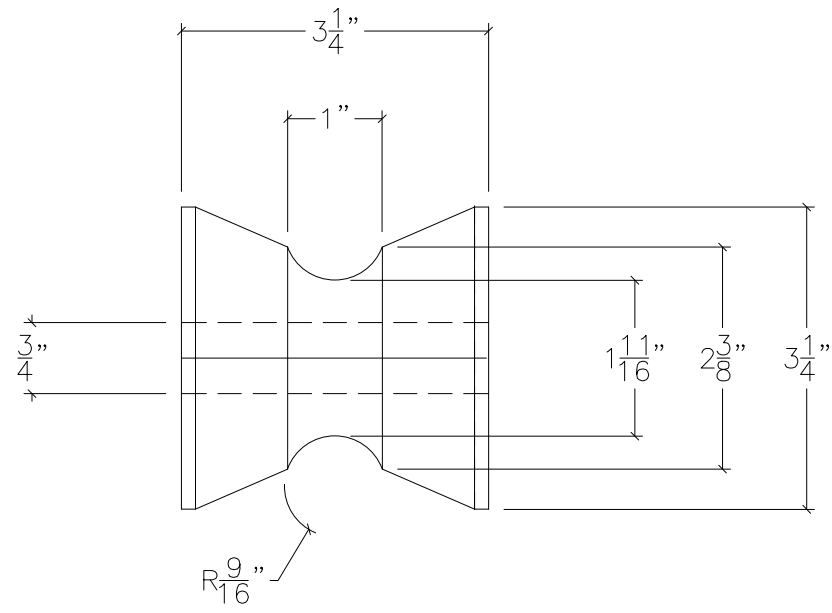
ROLLER #1
