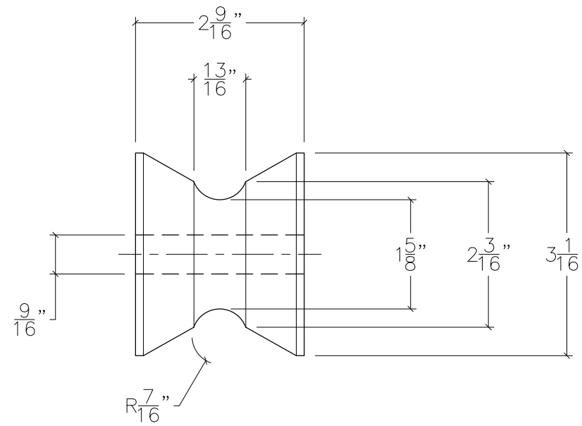
ROLLER #1
